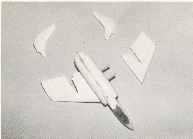
FIG. 10. Here the fuselage, wing, and vertical stabilizers are ready for final assembly. Mount the wing halves now, but hold off on the vertical stabilizers until you've installed the canopy.
