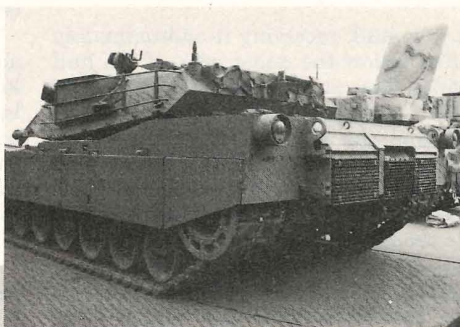
(Above) These close-ups show the drive sprocket and track detail, the grilled exhaust ports, and the folded wind sensor and canvas webbing on the rear of the turret.
