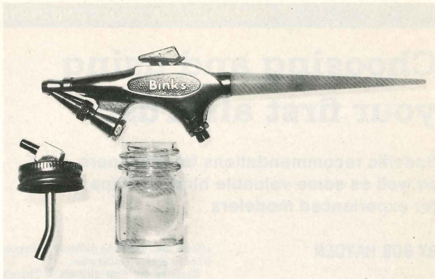
FIG. 2. This single-action, external mix Binks Wren "B" is one of three simple airbrushes recommended for beginners. This type is easy to use and easy to clean.
