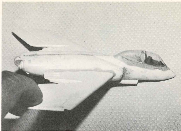
FIG. 11. Trim the canopy, attach with white glue, seal the seam with white glue, paint the seam with gray paint, and apply putty until the canopy fairs smoothly into the fuselage.
