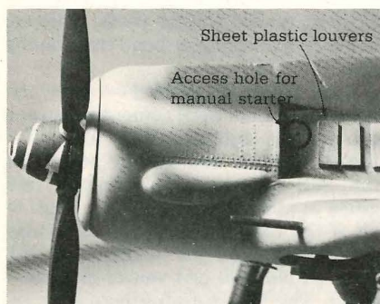
FIG. 9. Drill a small access hole for the manual starter crank on the left side, remove the molded louvers, and add sheet plastic louvers on both sides.
