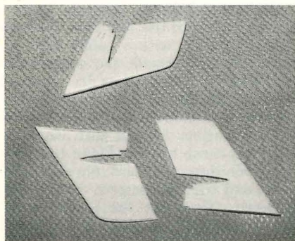
FIG. 8. In order to preserve detail on the outer surfaces, sand only the inside portions of the wing parts. Sand carefully until the trailing edge is sharp and the airfoil is symmetrical.
