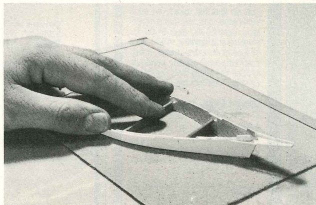
FIG. 3. After cutting the bottom portion of the model away, the waterlined hull must be smoothed. This boat hull has been reinforced with bulkheads of .090" ABS so that the sides won't deflect as the hull is rubbed over a sheet of coarse sandpaper.
