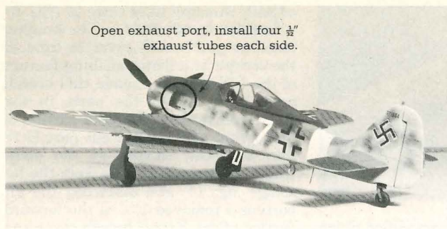
FIG. 7. Continue the conversion by improving the molded exhaust ports on the Monogram kit.
