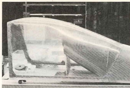
(Above) FIG. 2. The sliding portion of the FW-190F-8 canopy in the NASM restoration shop. (Left) FIG. 3. Close-up of the canopy, looking aft. The headrest is red, other parts are black-gray.
