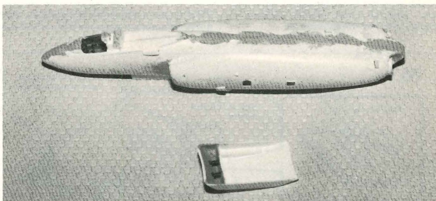
FIG. 7. Build by subassemblies (two shown here), filling all seams as you go.
