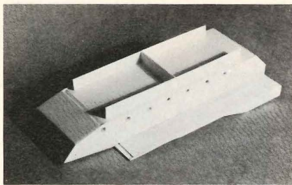
FIG. 7. The hull, upside down, with the spacer used to align the suspension.
