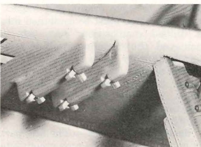
FIG. 14. Wing bomb racks with bomb shackles go just outboard of the main landing gear struts.
